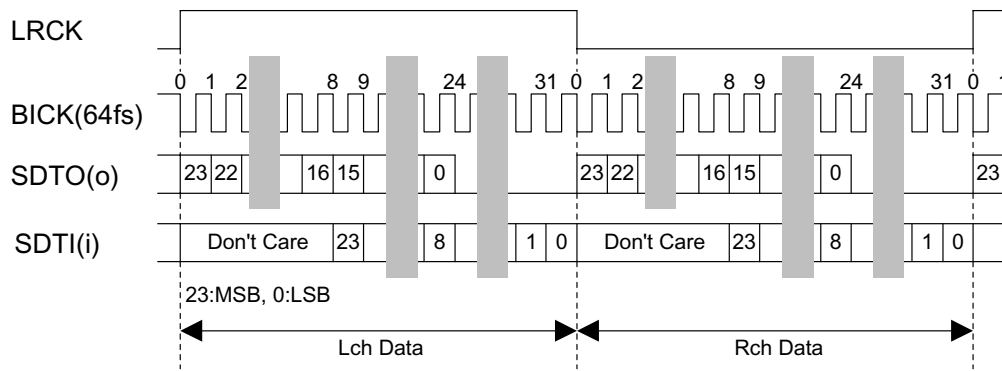
Figure 15. Mode 4 Timing
